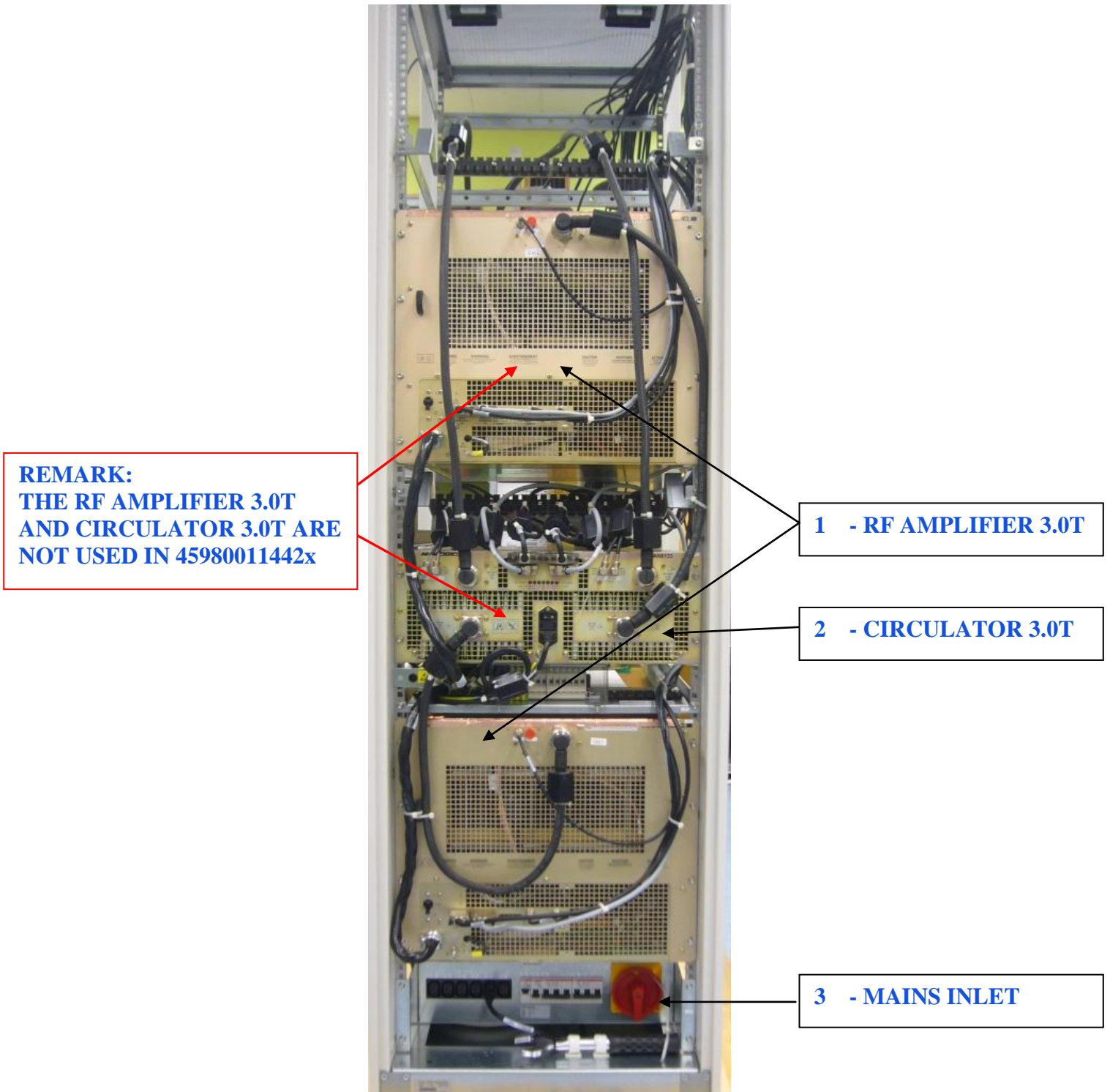
Figure 1 Frontview ACC cabinet
