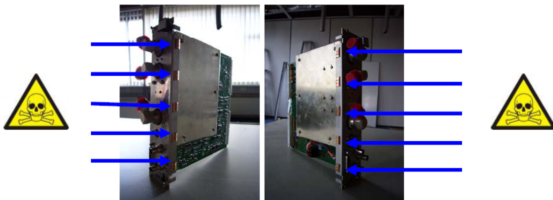
Figure 2, Beryllium Sticky-Fingers on Printed circuit board assembly
