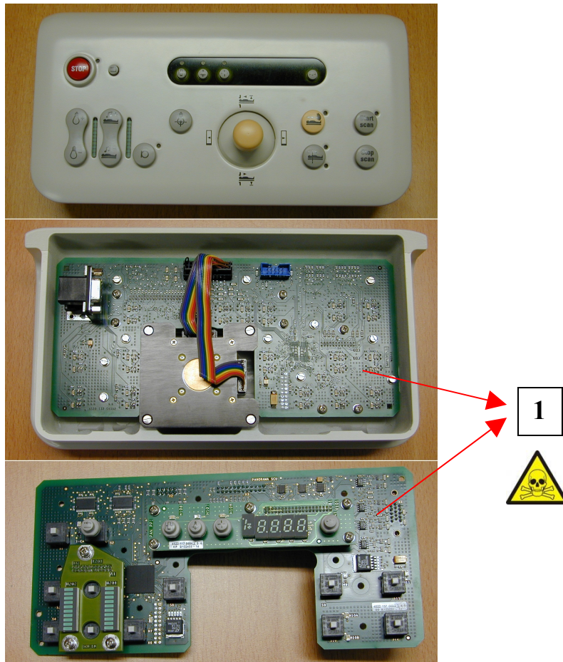
Figure 1: System Control Unit
