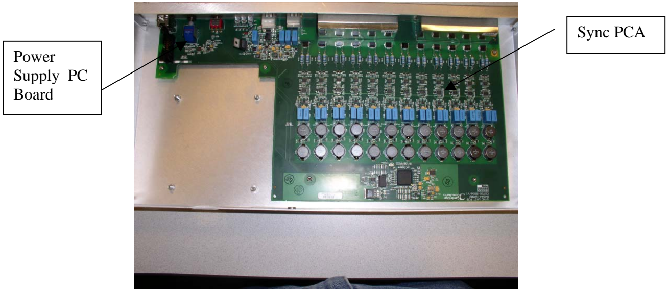
Figure 1 Sync PC Boards
