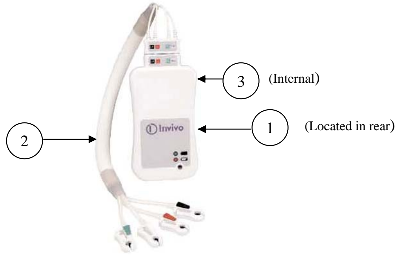
Figure 6: WECG Module with ECG Leads (Invivo Part Nos. 9312 and 9224)
