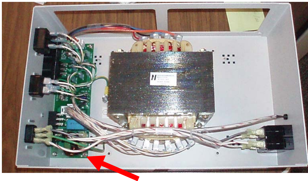
Figure 2 (Printed Circuit Card on one end of assembly)
