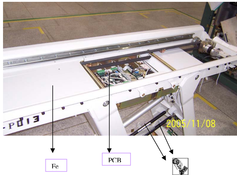
Figure 8 Couch (inside view)
