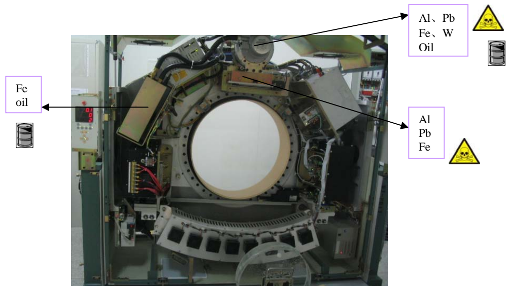
Figure 2 Gantry front view (without cover)
