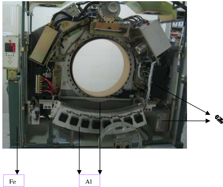
Figure 3 Gantry front view (without cover)
