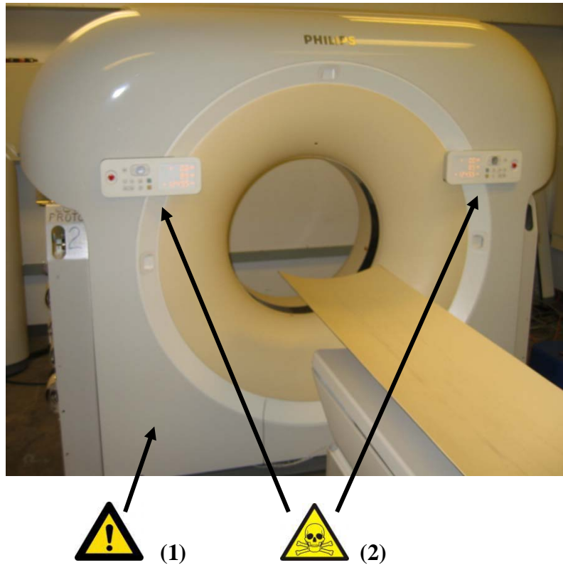
Figure 1: Front View of Gantry with Covers on
