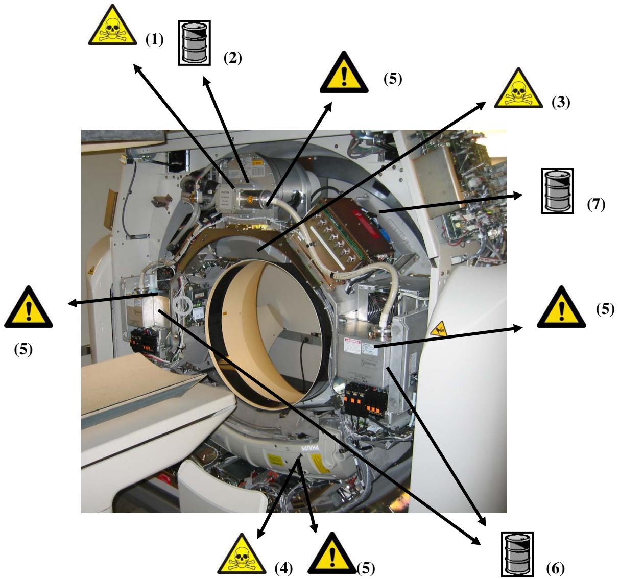
Figure 3: Front View of Gantry with Front Cover Lifted
