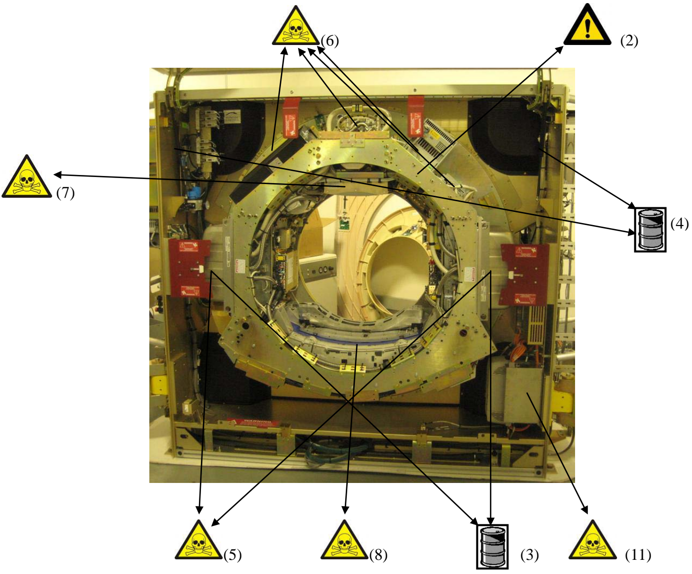
Figure 2: Front View of Gantry with Front Cover Raised
