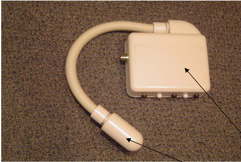
Figure 1 7T Linear T/R interface box.
