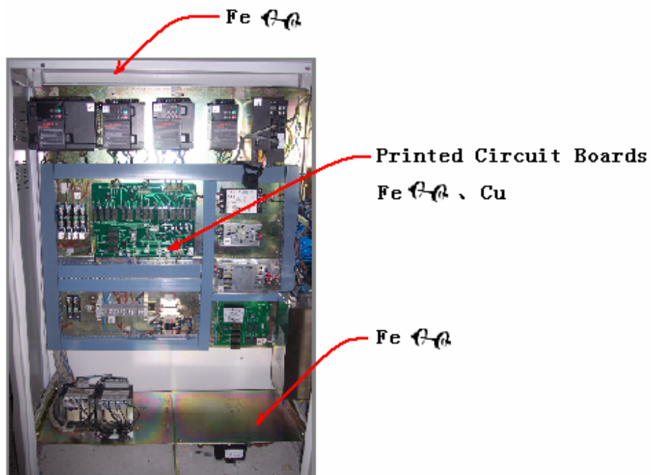
Fig 4 Power control cabinet
