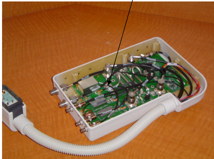
Figure 2. 7T Achieva TR Interface box, opened view.
