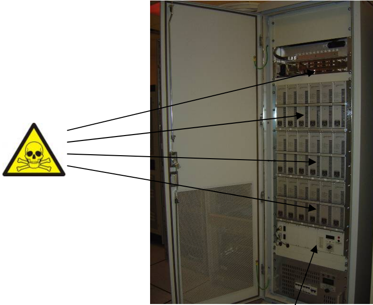
Figure 1. 7T Shim cabinet, front view.
