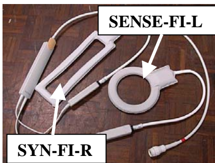
Flex-R IT & Flex-L IT coils
