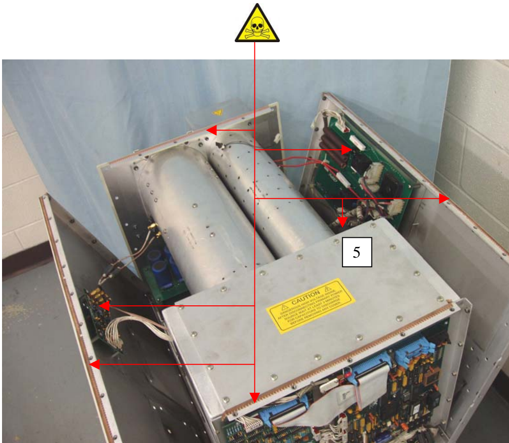
Figure 3 RF Deck – Top View Sides Open
