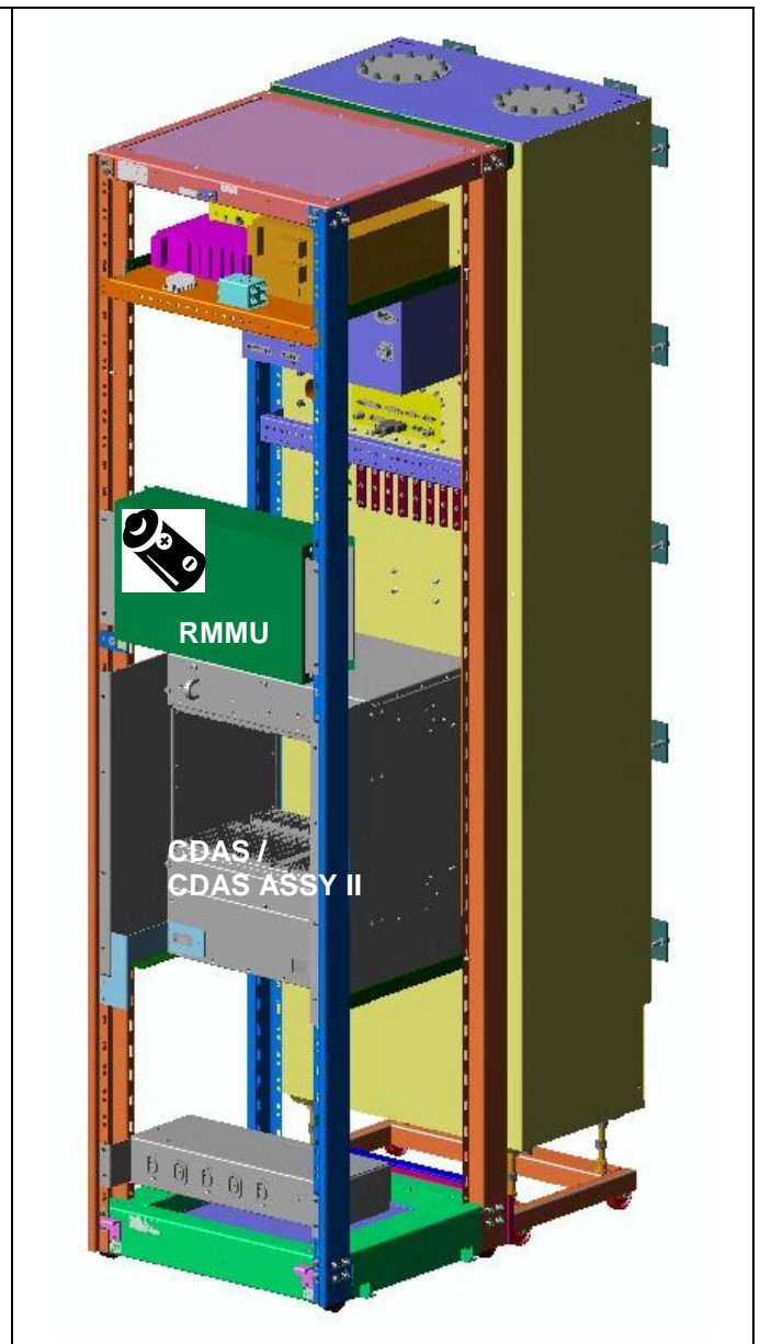
Figure 2: FCC seen from Technical room side
