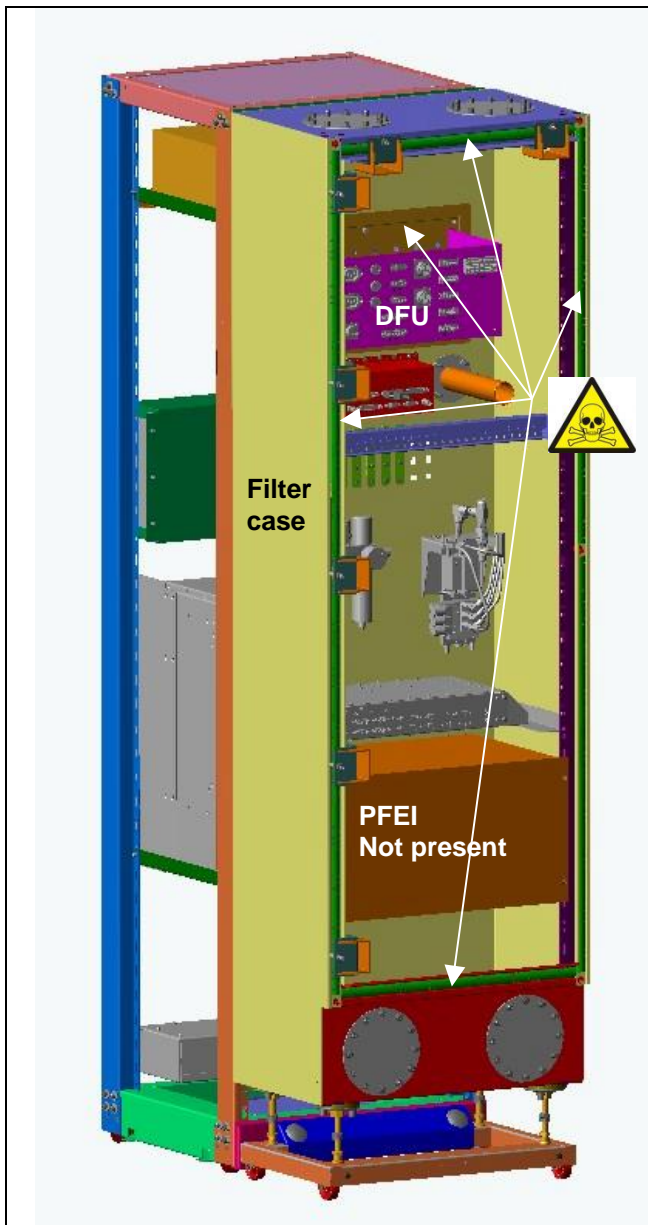
Figure 1: FCC seen from Scanner room side
