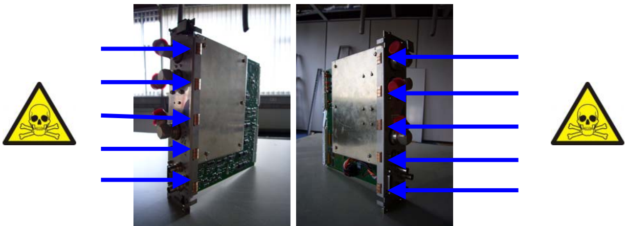
Figure 2, Beryllium Sticky-Fingers on Printed circuit board assembly Recycling Passport Revision History
