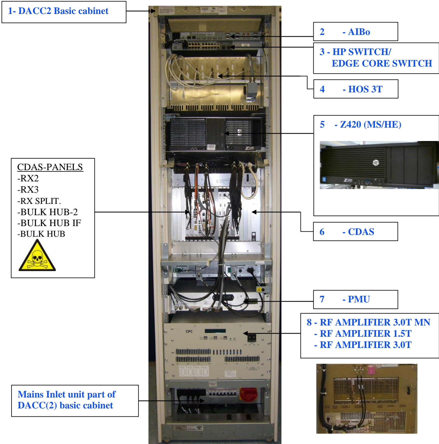
Figure 1 Frontview DACC2 cabinet
