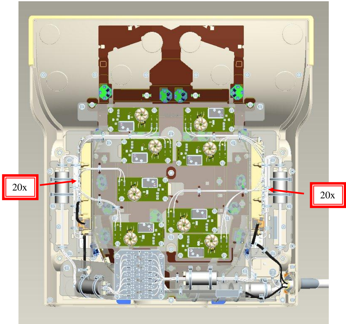
Figure 3, SMP Connector (multiple locations) in NVC Base 1.5T
