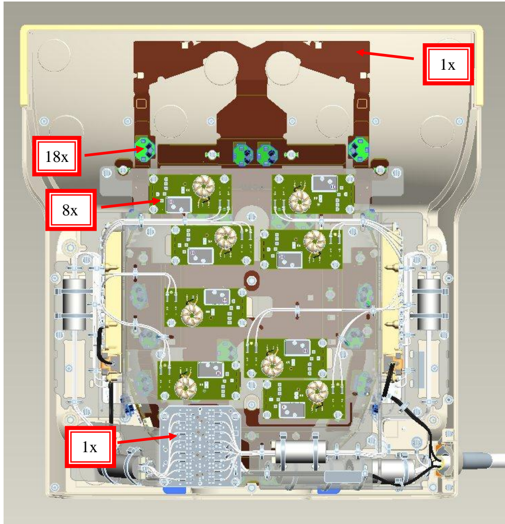
Figure 1, NVC Base 1.5T pcb locations
