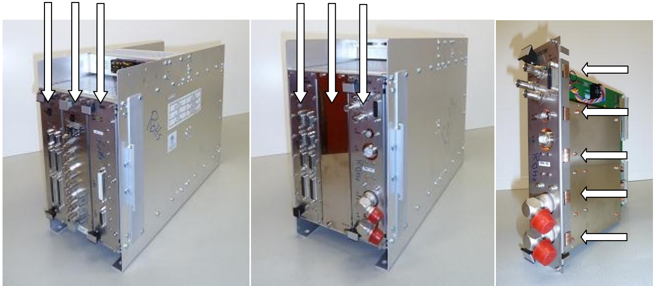
Figure 1, PCB-Assemblies in the front and back of the PFEI-DDAS unit and the position of the Sticky-Fingers on the PCB-Assembly
