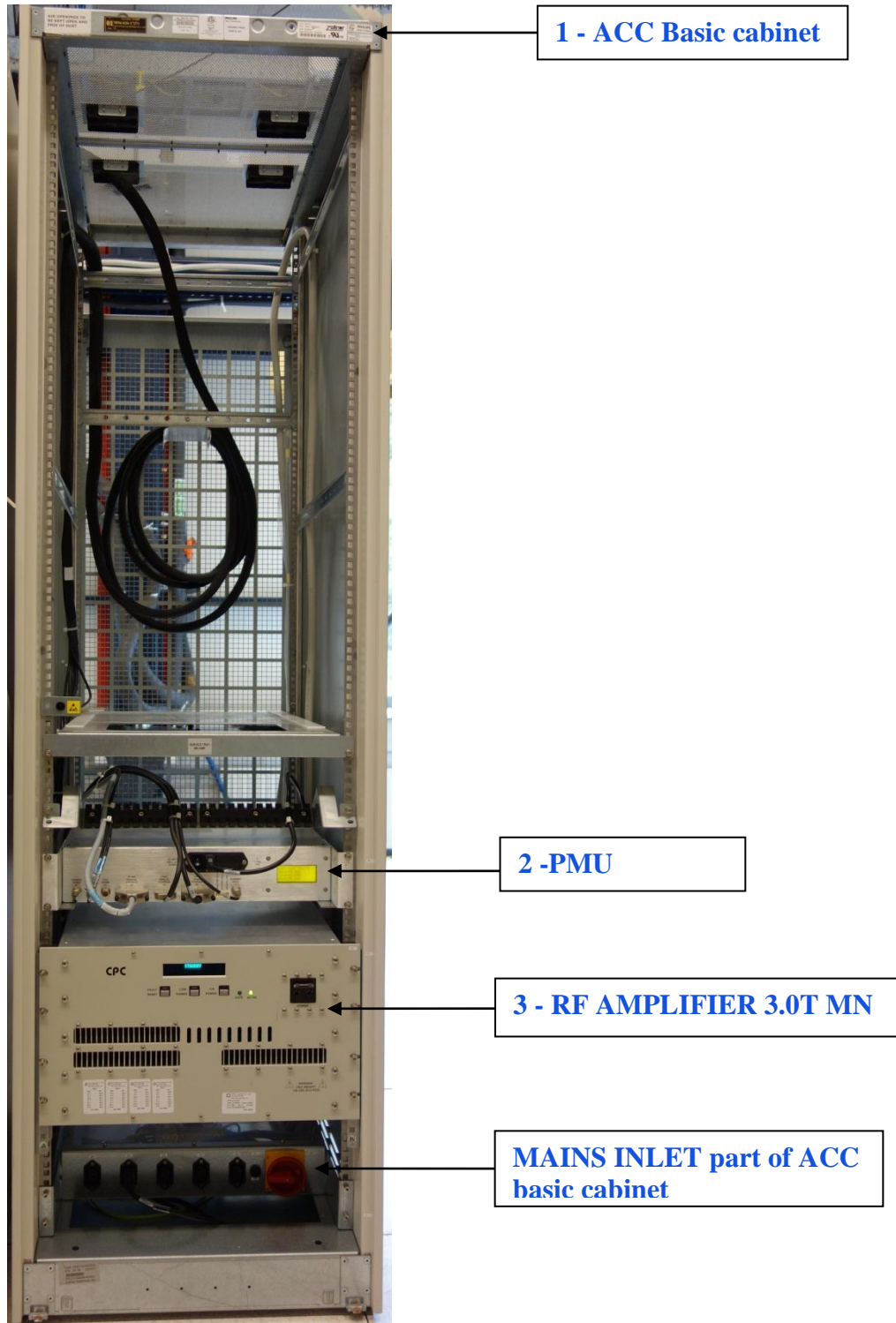
Figure 1 Frontview ACC cabinet
