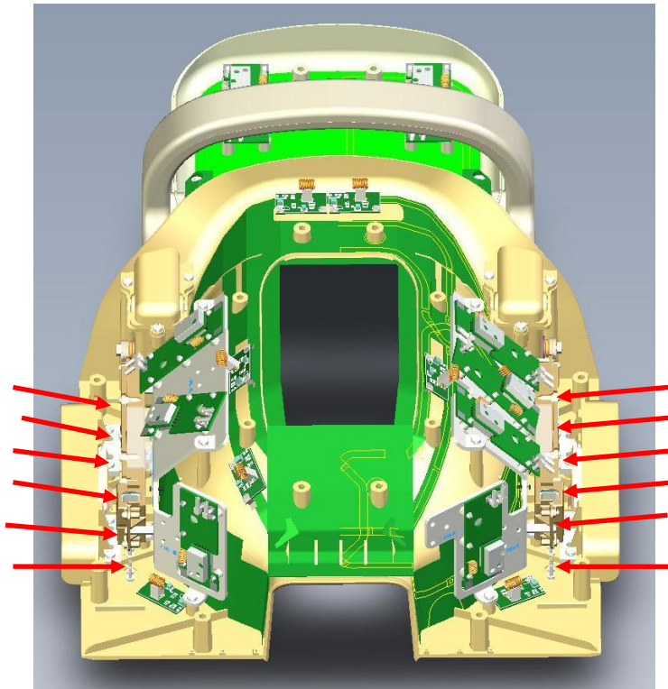
Figure 3, NVC Head Neck 1.5T contact pin locations (protruding bottom cover)
