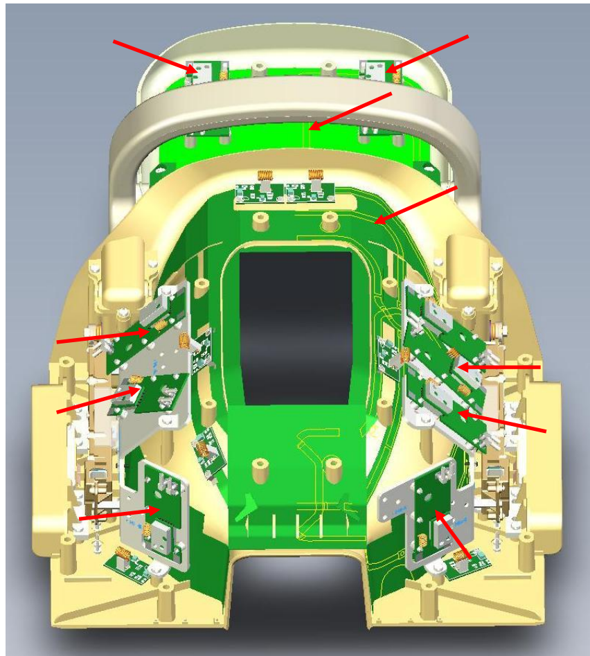
Figure 1, NVC Head Neck 1.5T pcb locations
