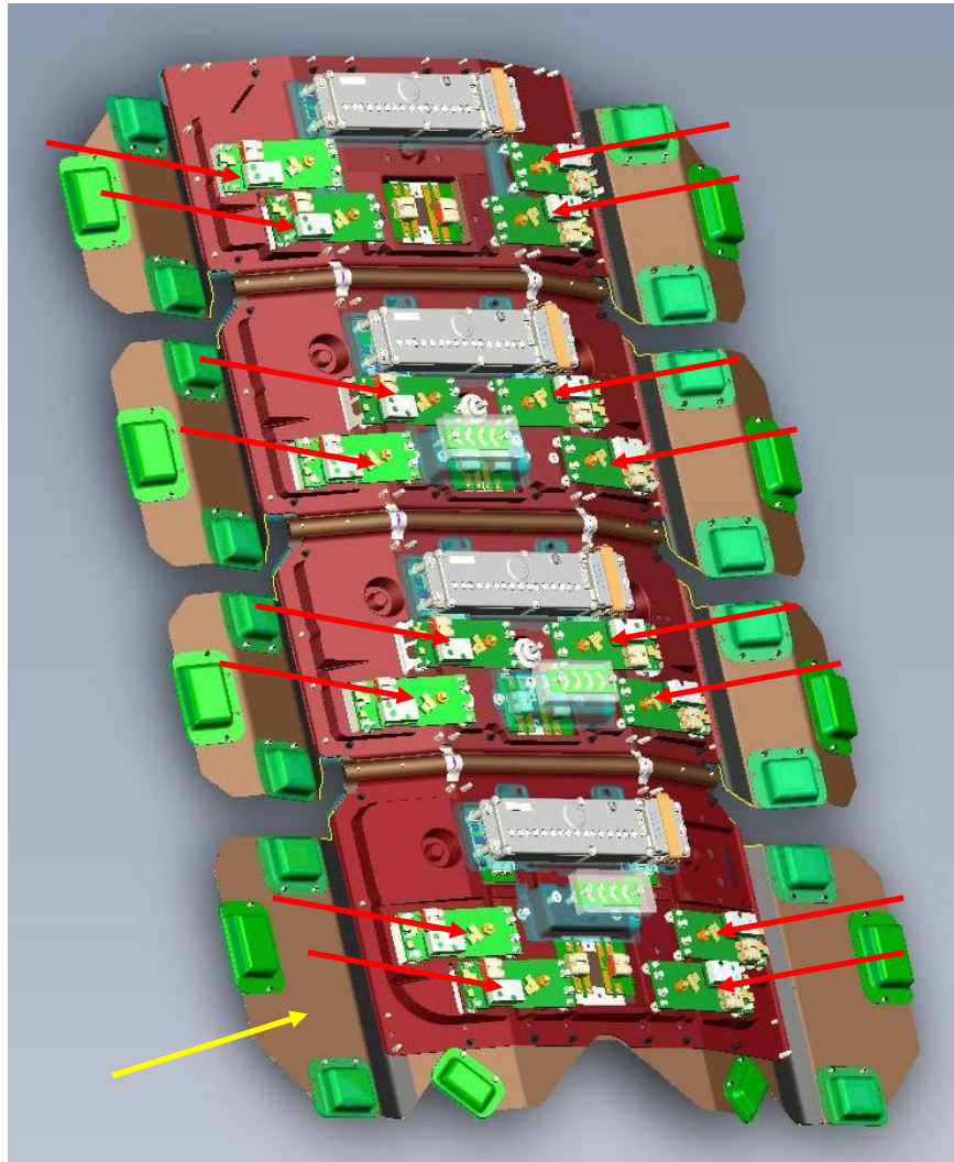
Figure 1. Anterior Coil M2 1.5T pcb locations
