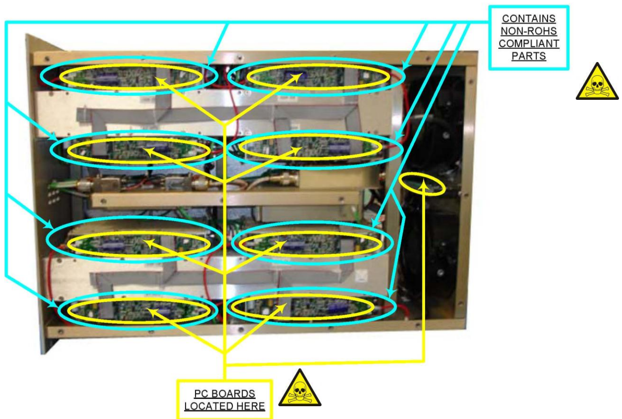
7T4KMP POWER AMP – TOP VIEW
