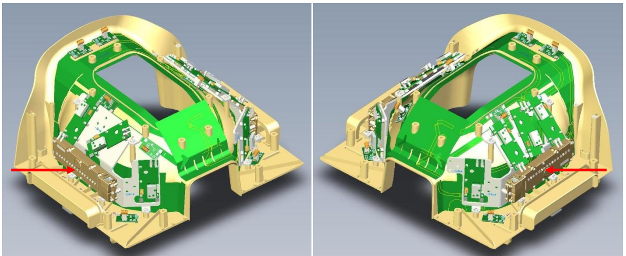
Figure 2a, 2b, NVC Head 1.5T RXE locations
