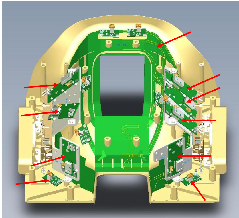
Figure 1, NVC Head 1.5T pcb locations
