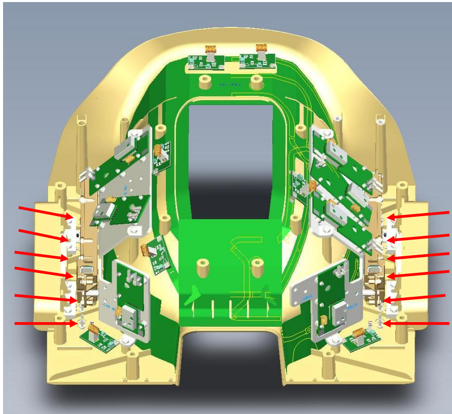
Figure 3, NVC Head 1.5T contact locations (protruding bottom cover)
